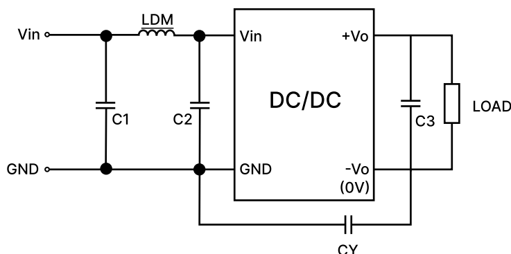
Figure 2: EMC Typical Recommended Circuits
