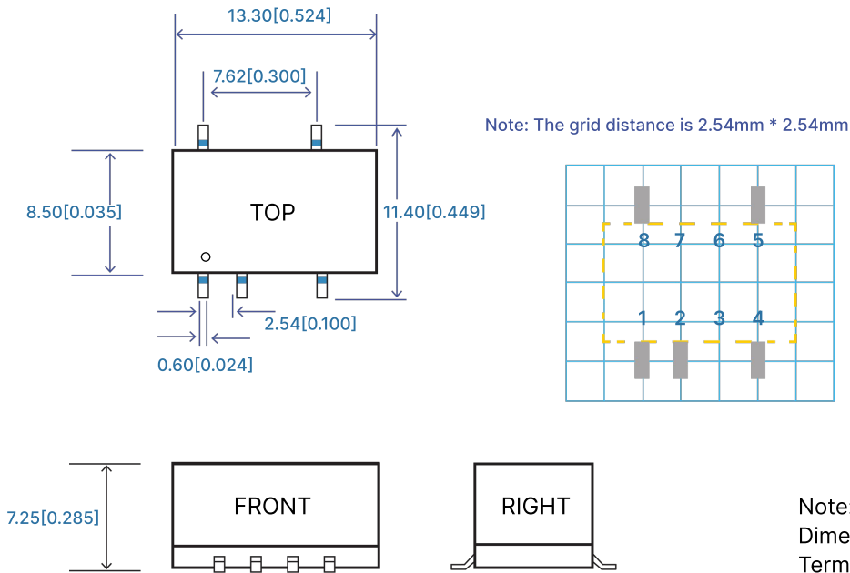
Figure 7: Overall dimensions
