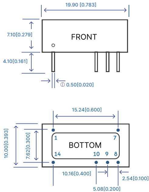
Figure 7: Overall dimensions
