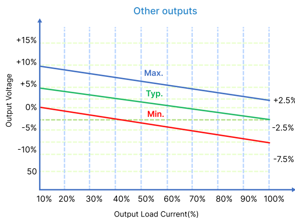
Figure 3: Voltage tolerance envelope
