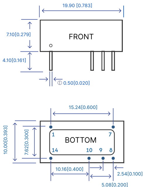
Figure 7: Overall dimensions
