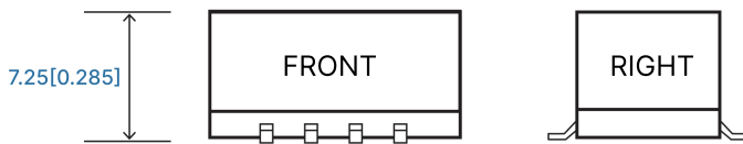
Figure 7: Overall dimensions
