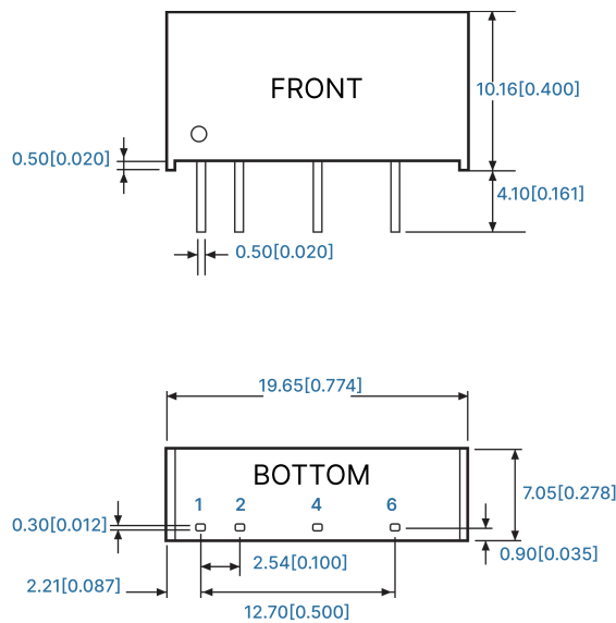
Figure 7: Overall dimensions
