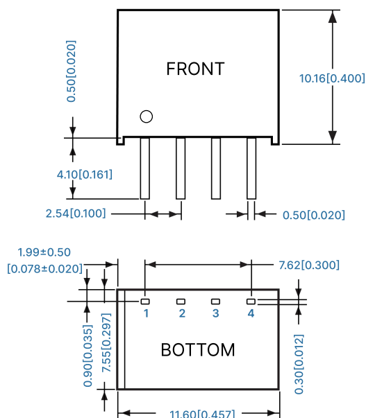
Figure 7: Overall dimensions
