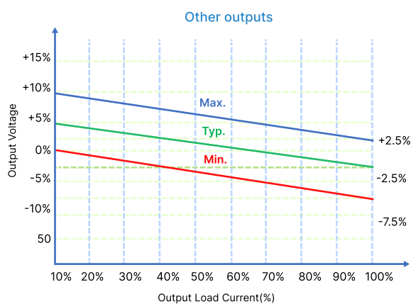
Figure 3: Voltage tolerance envelope
