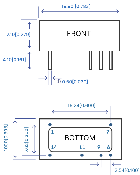
Figure 7: Overall dimensions
