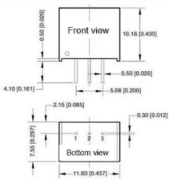
Figure 7: Overall dimensions
