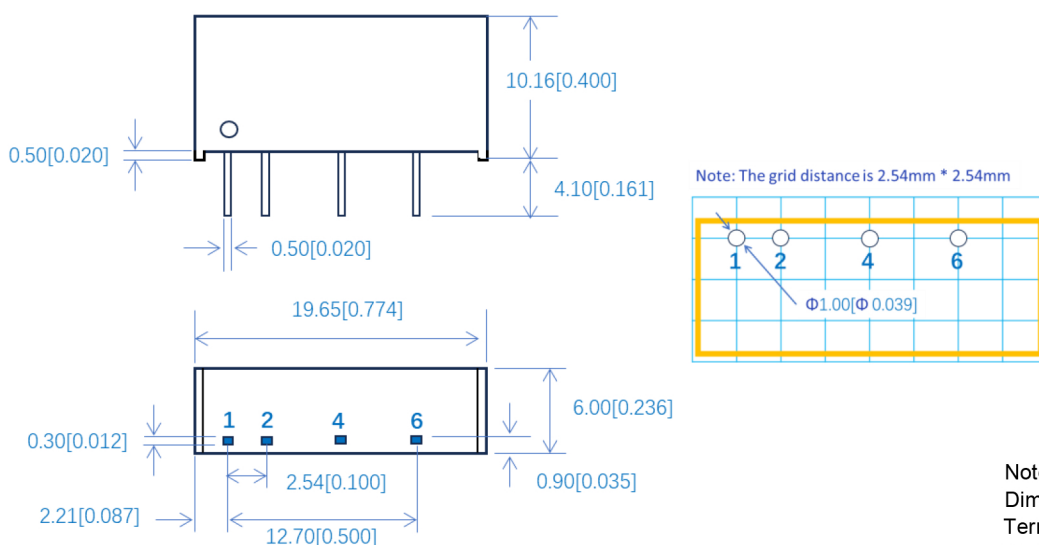
Figure 7: Overall dimensions
