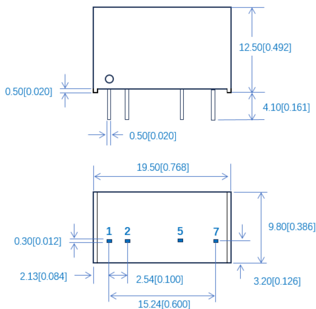
Figure 7: Overall dimensions
