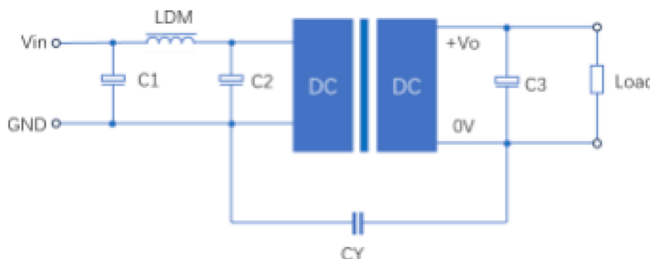
Figure 2: EMC Typical Recommended Circuits
