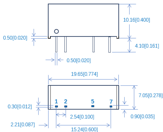
Figure 7: Overall dimensions
