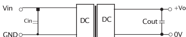
Figure 1: Application circuit
