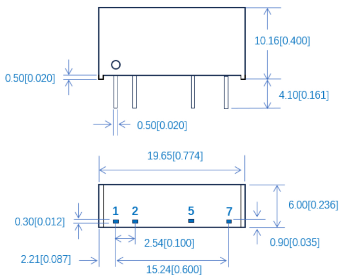
Figure 7: Overall dimensions
