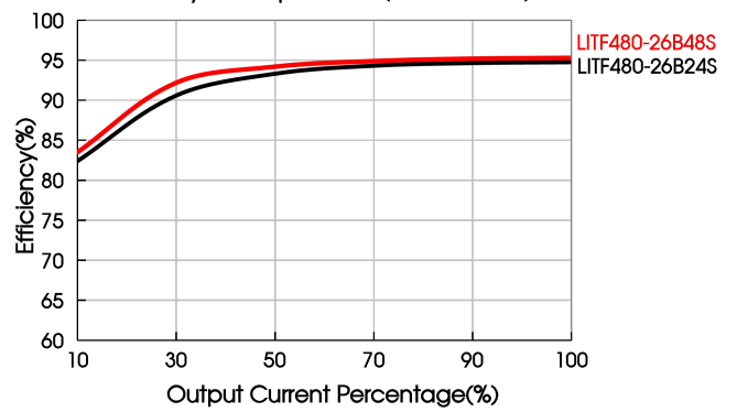
Efficiency Vs Output Load (Vin=400VAC)
